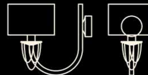
4361/A Бра L275xH180xSP323 E14 1*60W IP 20
